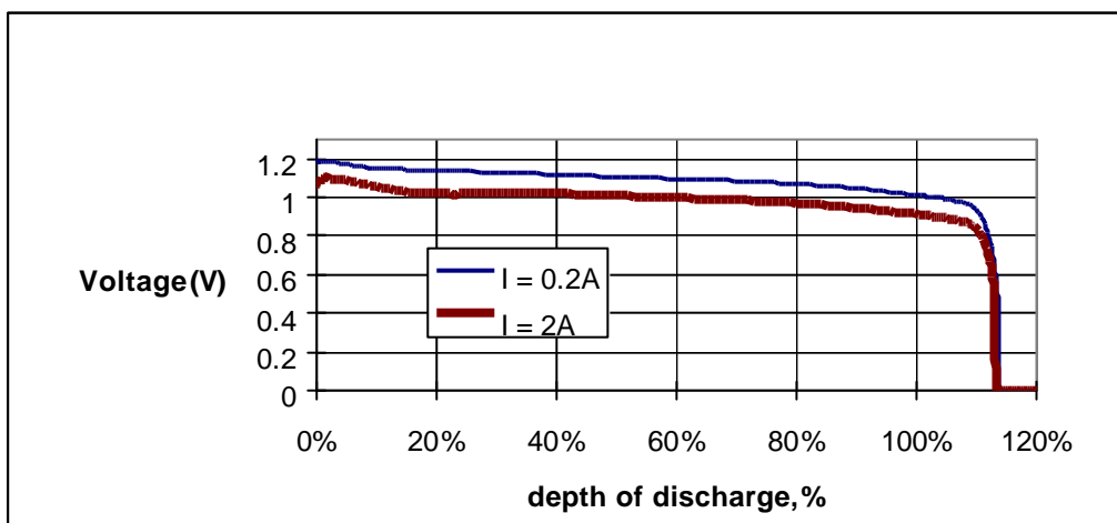
Figure 4. Cell voltages during GSM discharge, as a function of depth of discharge, 0.2A / 2A GSM regime
