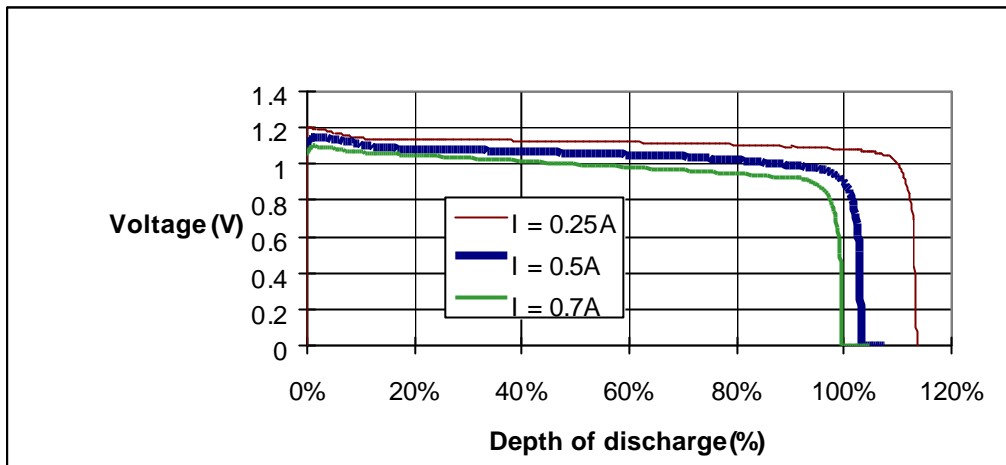
Figure 3. Cell voltages during constant-current discharge, as a function of depth of discharge, for three different current values.
