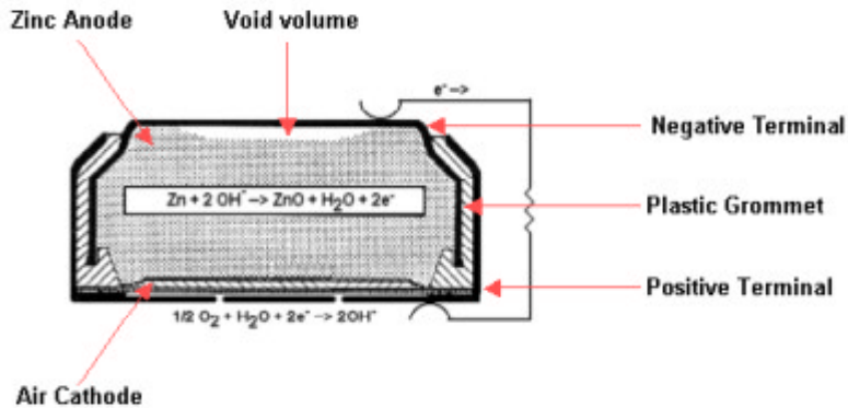
Figure 1. Schematic of zinc -air cell
