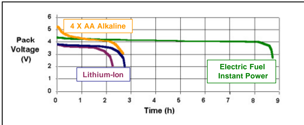
Figure 7. Comparison of GSM-mode talk time
