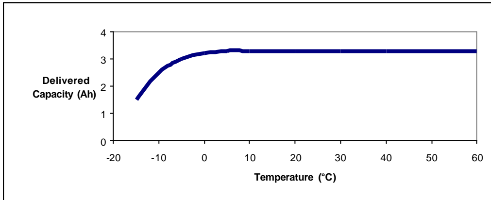
Figure 5. Cell capacity as a function of ambient temperature
