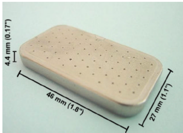
Figure 2. Photograph and dimensions of 3300 mAh zinc -air cell
